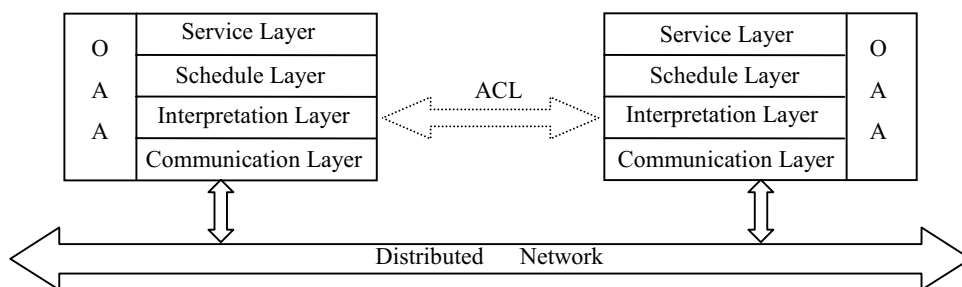
Figure 3. The structure model of OAA
