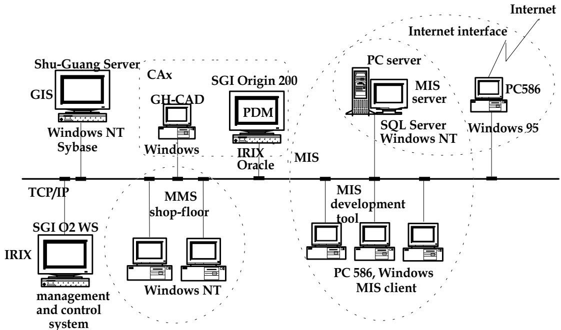
Fig. 8 The MACIP Develop Environment
