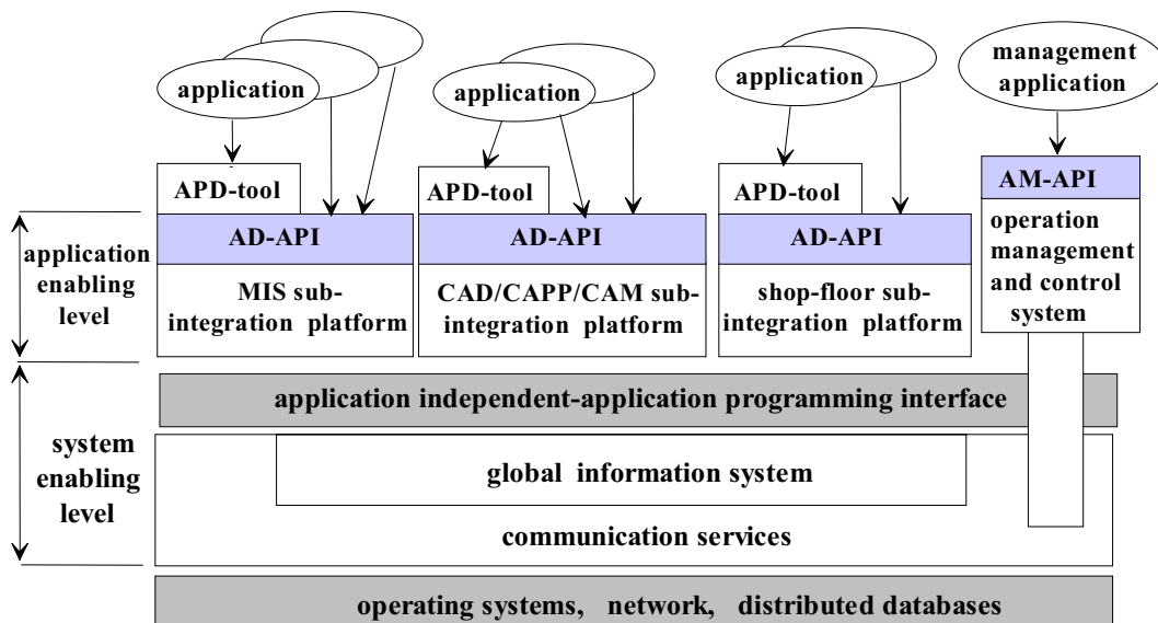
Fig. 3 MACIP system architecture
