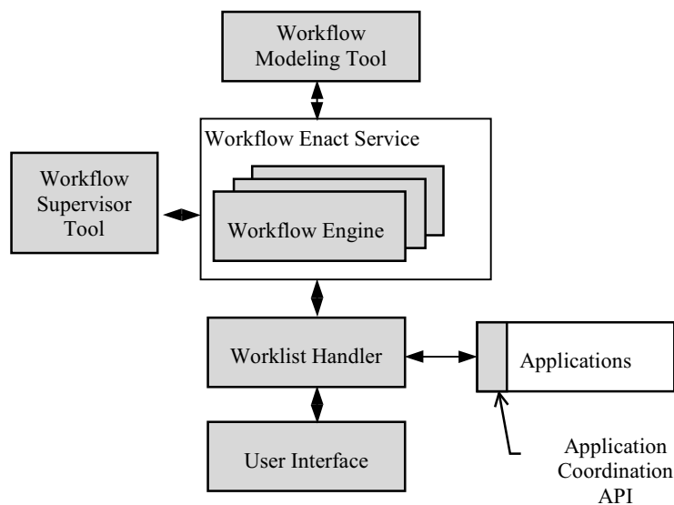
Fig. 12 Workflow Management Module structure
