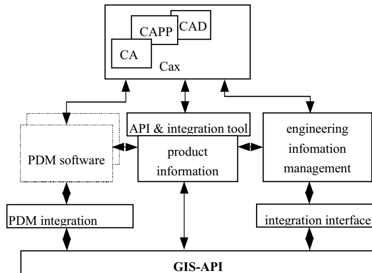
Fig. 5 CAD/CAPP/CAM SIP structure
